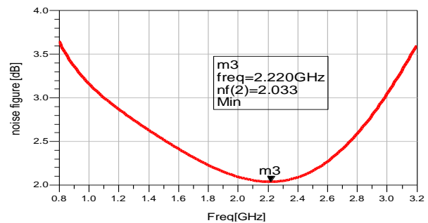
Fig. 8 Noise Figure of LNA
