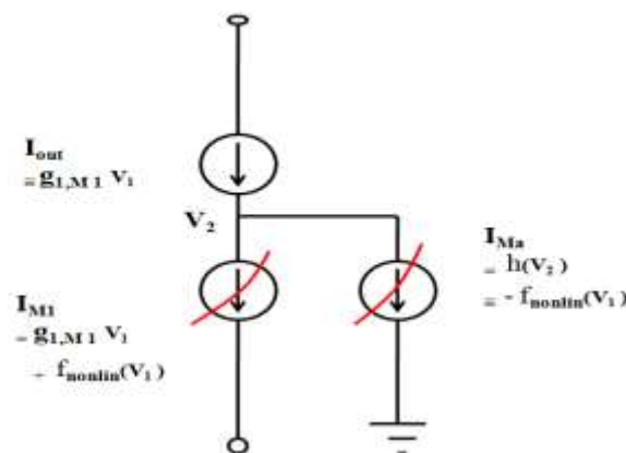
Fig. 3 Conceptual view of the proposed linearization technique
