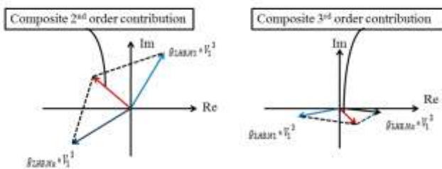
Fig. 4 Vector diagram of the proposed technique for the IM3 products
