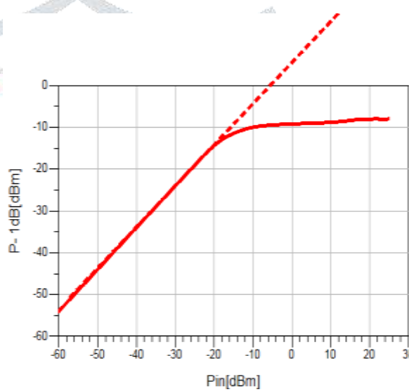
Fig. 10 “1-dB” compression point of LNA
