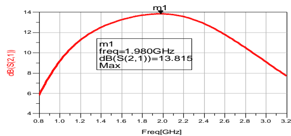
Fig. 6 Gain of LNA
