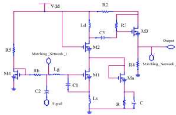
Fig. 1 Complete Schematic of proposed L-deg common source CascodeLNA
