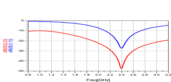
Fig.5 Input and output reflection coefficient of LNA
