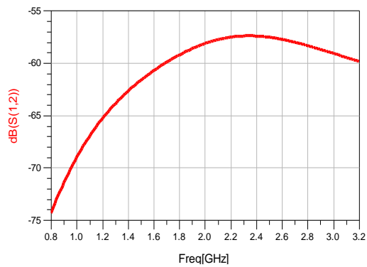
Fig. 7 Reverse Isolation of LNA
