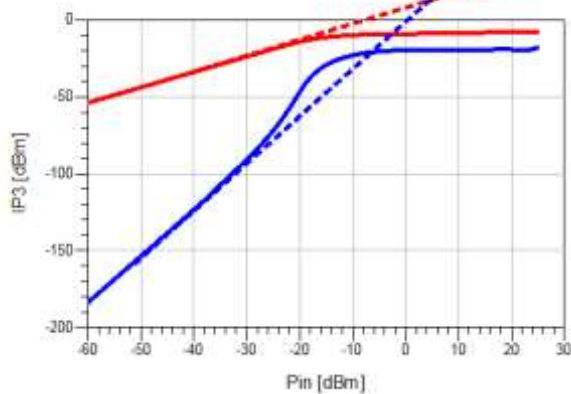
Fig. 9 IIP3 of LNA
