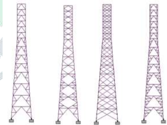
Fig 1:-bracing pattern (K, XB, W, V - Type)
