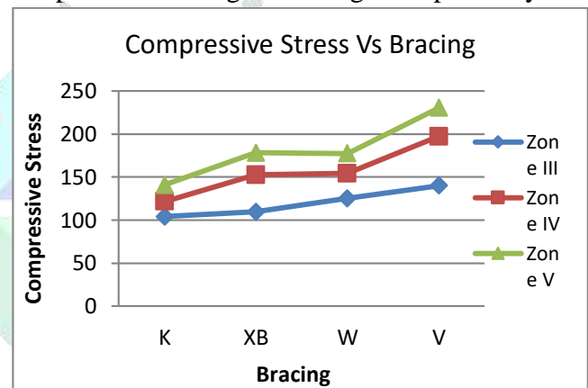
Fig.6: Compressive stress vs bracing
