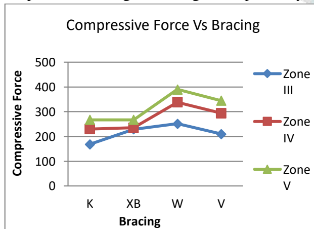
Fig.4: Compressive force vs bracing
