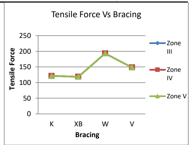
Fig.5: Tensile force vs bracing
